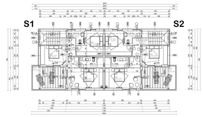
1. KAT - 1st FLOOR - 1.OBERGESCHOSS
